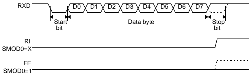
Figure 9-2. UART Timings in Mode 1
