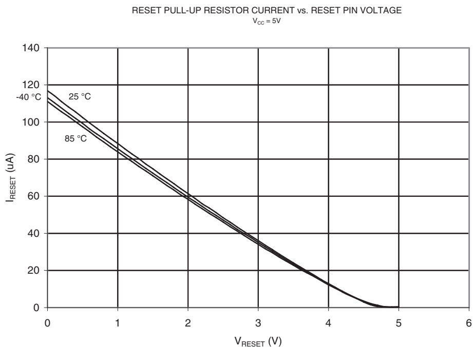
Figure 19-17. Reset Pull-up Resistor Current vs. Reset Pin Voltage ( V_{CC} = 5V )
