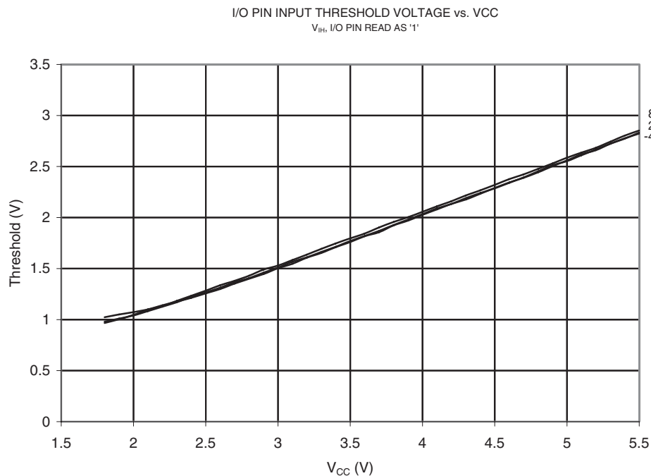
Figure 19-33. I/O Pin Input Threshold Voltage vs. V_{CC} ( V_{IH} , I/O Pin Read as '1')
