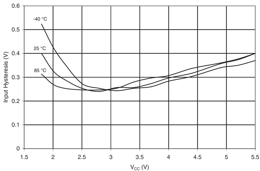
Figure 19-36. Reset Pin as I/O - Input Threshold Voltage vs. V_{CC} ( V_{IH} , Reset Pin Read as '1')
