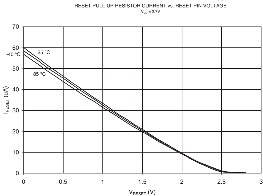
Figure 19-18. Reset Pull-up Resistor Current vs. Reset Pin Voltage ( V_{CC} = 2.7V )
