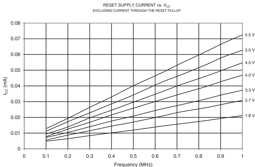
Figure 19-59. Reset Supply Current vs. V_{CC} (0.1 - 1.0 MHz, Excluding Current through the Reset Pull-up)
