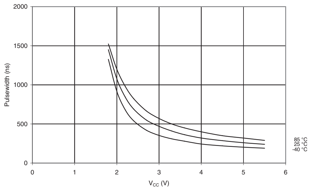
Figure 19-61. Reset Pulse Width vs. V_{CC}
