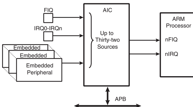
Figure 23-1. Block Diagram
