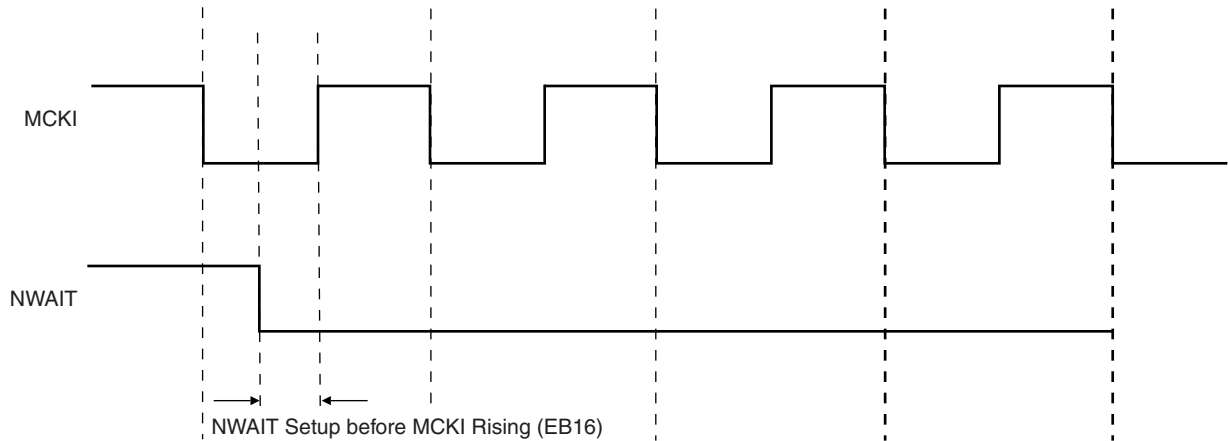
Figure 24-1. NWAIT Rising
