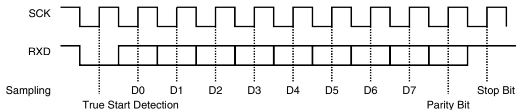
Figure 17-5. Synchronous Mode: Character Reception
