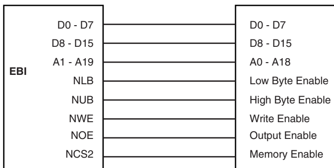
Figure 11-5. Memory Connection for a 16-bit Data Bus
