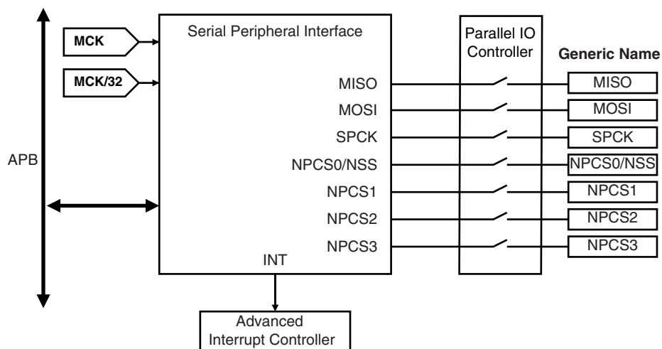
Figure 19-1. SPI Block Diagram
