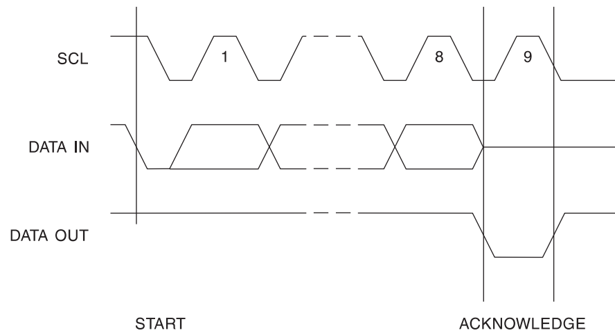
Figure 8-5. Output Acknowledge
