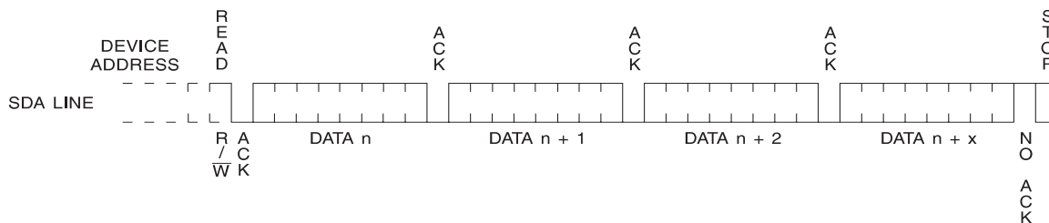
Figure 8-5. Sequential Read
