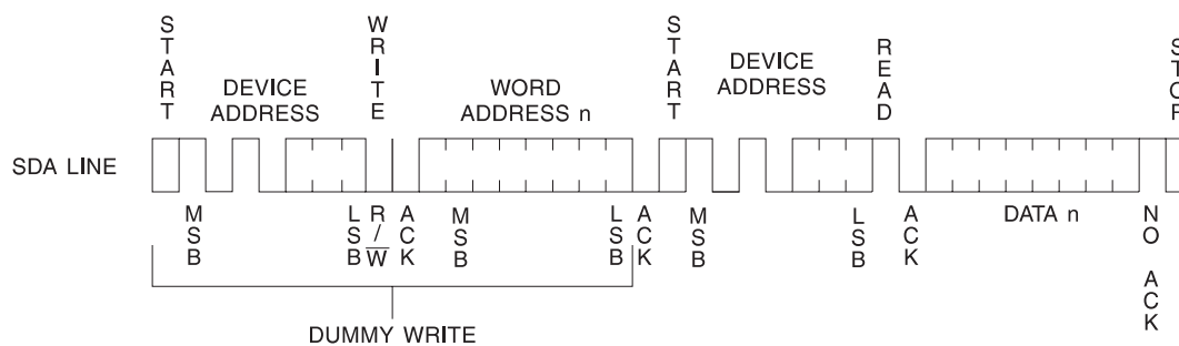
Figure 8-4. Random Read
