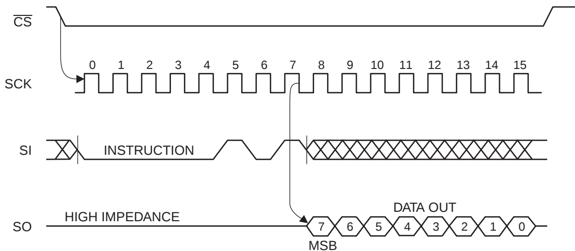
Figure 6. RDSR Timing
