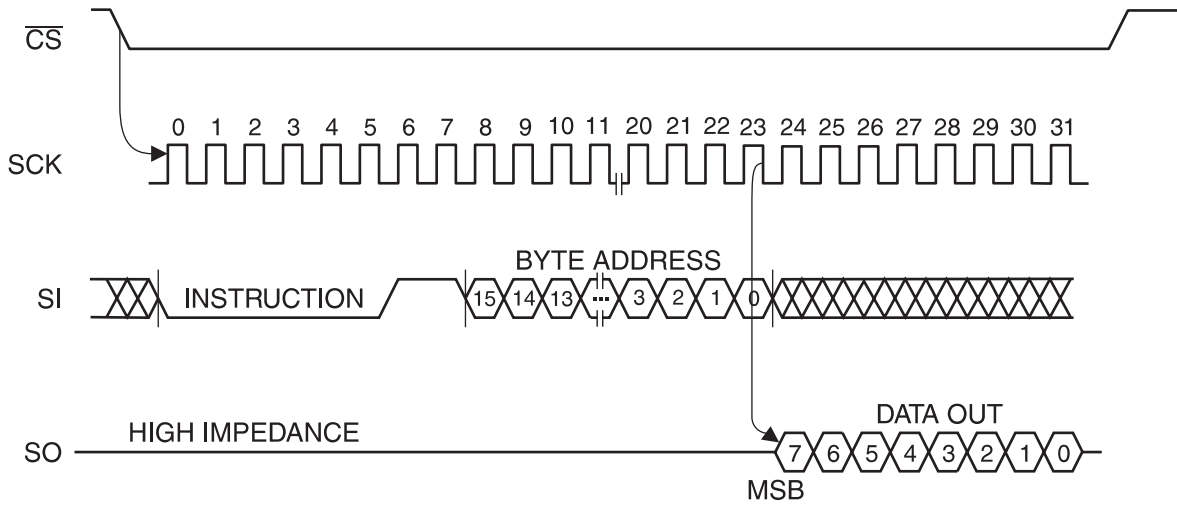
Figure 8. READ Timing
