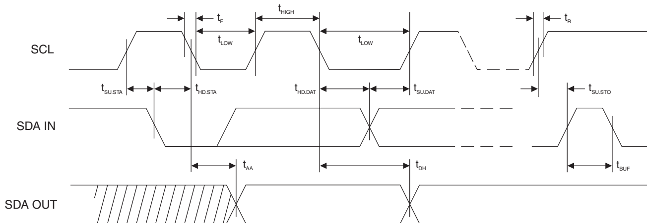
Figure 5-4. Bus Timing
