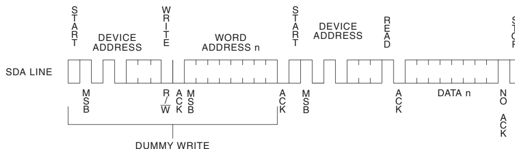
Figure 8-2. Random Read
