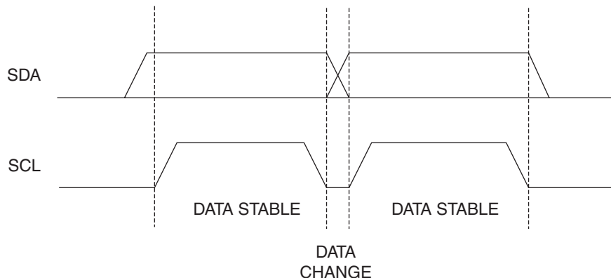
Figure 5-1. Data Validity
