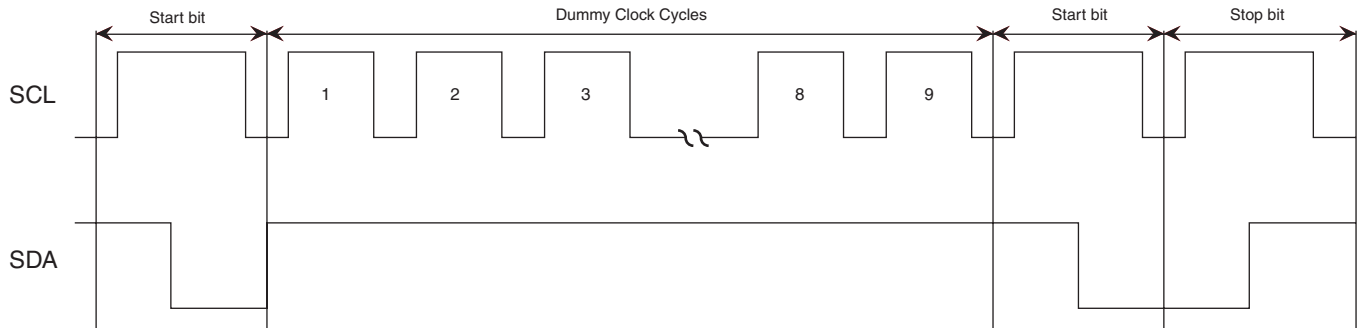
Figure 5-4. Bus Timing
