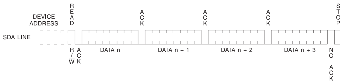
Figure 13-6. Sequential Read
