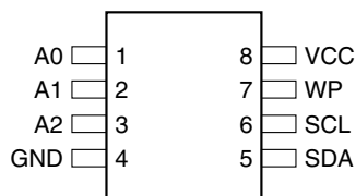
8-lead TSSOP
