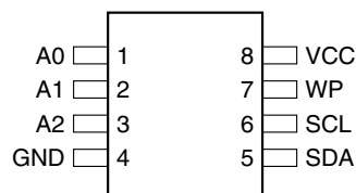
8-lead SOIC
