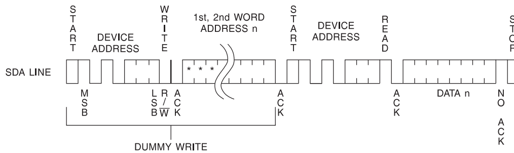
Figure 13-5. Random Read
