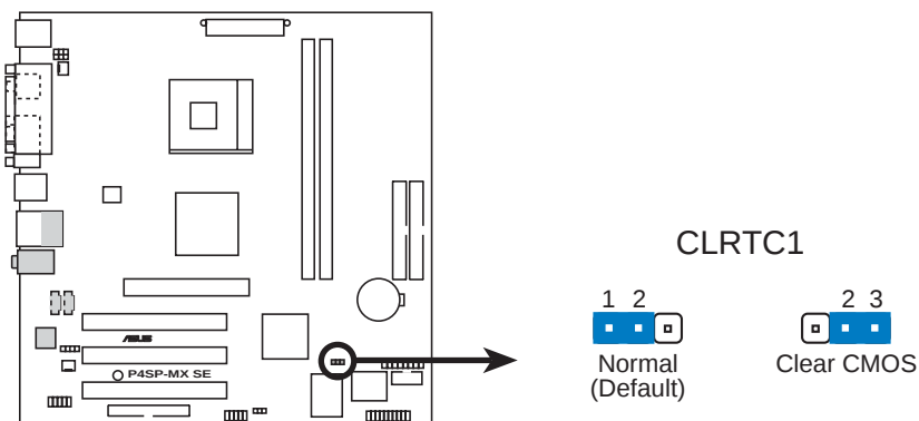
P4SP-MX SE Clear RTC RAM setting
