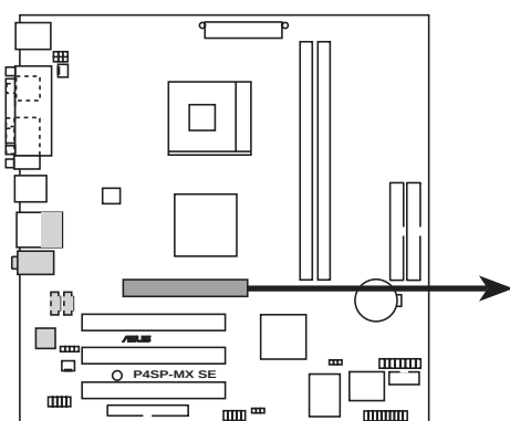
P4SP-MX SE Accelerated Graphics Port (AGP)
