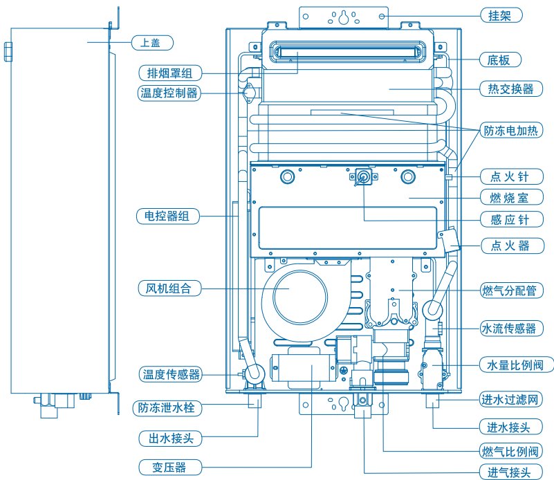
a. JSW48-Hi7/JSW40-Hi7/JSW48-Hi7S/JSW40-Hi7S机型:
