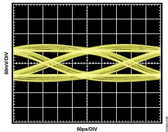
Figure 28. 3.75 Gbps Output Eye, 15 Meters CX4 Cable, PE = Best Setting (TP3 from Figure 24)
