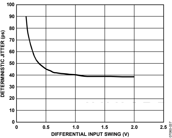
Figure 30. Deterministic Jitter vs. Differential Input Swing
