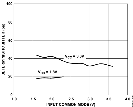
Figure 32. Deterministic Jitter vs. Input Common Mode
