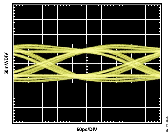
Figure 27. 3.25 Gbps Output Eye, 15 Meters CX4 Cable, PE = Best Setting (TP3 from Figure 24)
