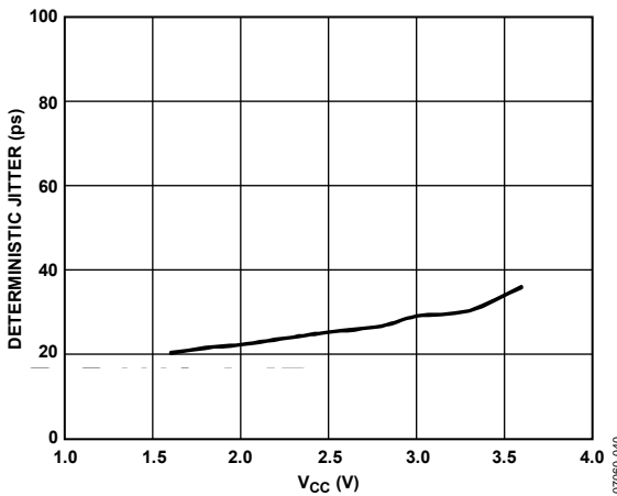
Figure 33. Deterministic Jitter vs. Supply Voltage
