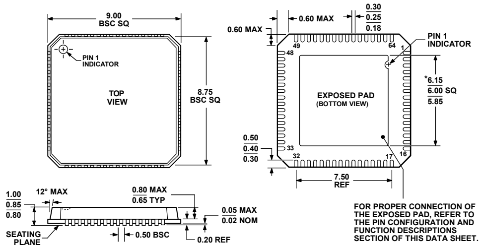
*COMPLIANT TO JEDEC STANDARDS MO-220-VMMD-4 EXCEPT FOR EXPOSED PAD DIMENSION Figure 44. 64-Lead Lead Frame Chip Scale Package [LFCSP_VQ] 9 mm x 9 mm Body, Very Thin Quad (CP-64-2) Dimensions shown in millimeters
