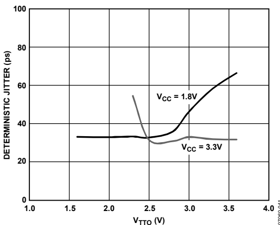
Figure 34. Deterministic Jitter vs. Output Termination Voltage
