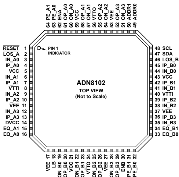
Figure 3. Pin Configuration
