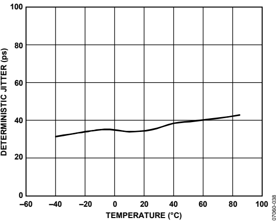
Figure 31. Deterministic Jitter vs. Temperature
