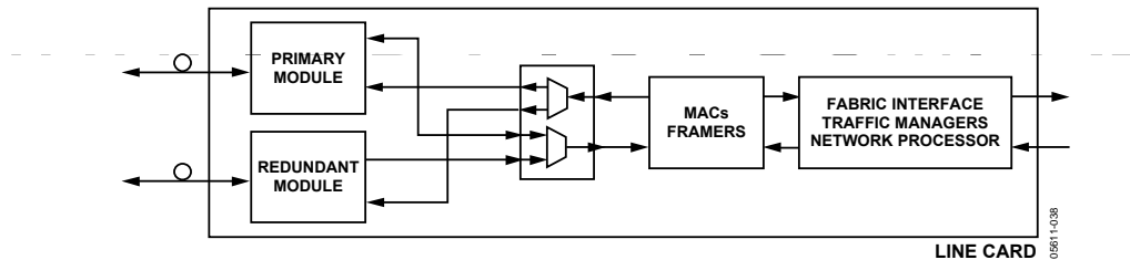
Figure 39. Using the AD8159 for Line Interface Redundancy
