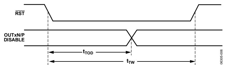
Figure 6. Asynchronous Reset
