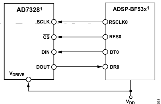
Figure 55. Interfacing the AD7328 to the ADSP-BF53x
