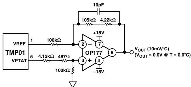
Figure 14. Translating 5 mV/K to 10 mV/°C
