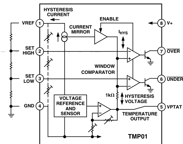
Figure 2. Detailed Block Diagram
