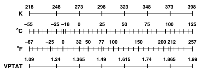
Figure 5. Temperature—VPTAT Scale
