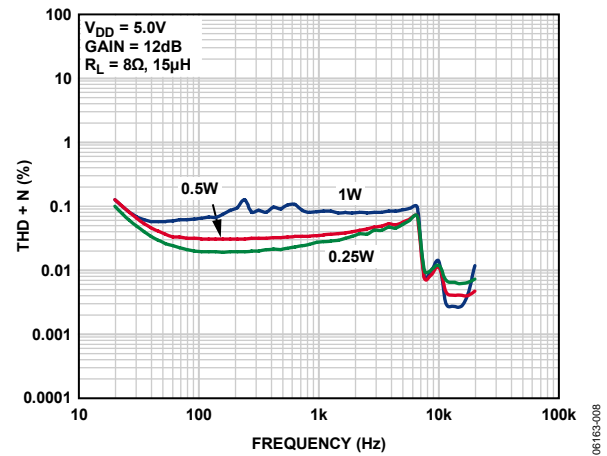
Figure 7. THD + N vs. Frequency, V_{DD} = 5.0V , A_v = 12dB , R_L = 8\Omega
