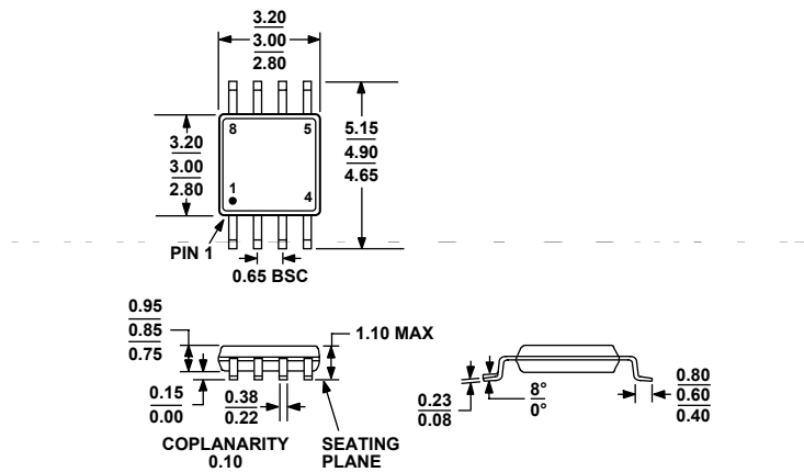
Figure 31. 8-Lead Mini Small Outline Package [MSOP] (RM-8) Dimensions shown in millimeters
