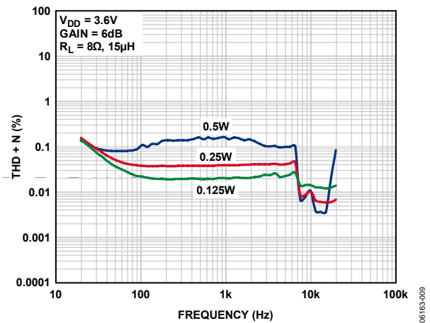
Figure 8. THD + N vs. Frequency, V_{DD} = 3.6V , A_v = 6dB , R_L = 8\Omega
