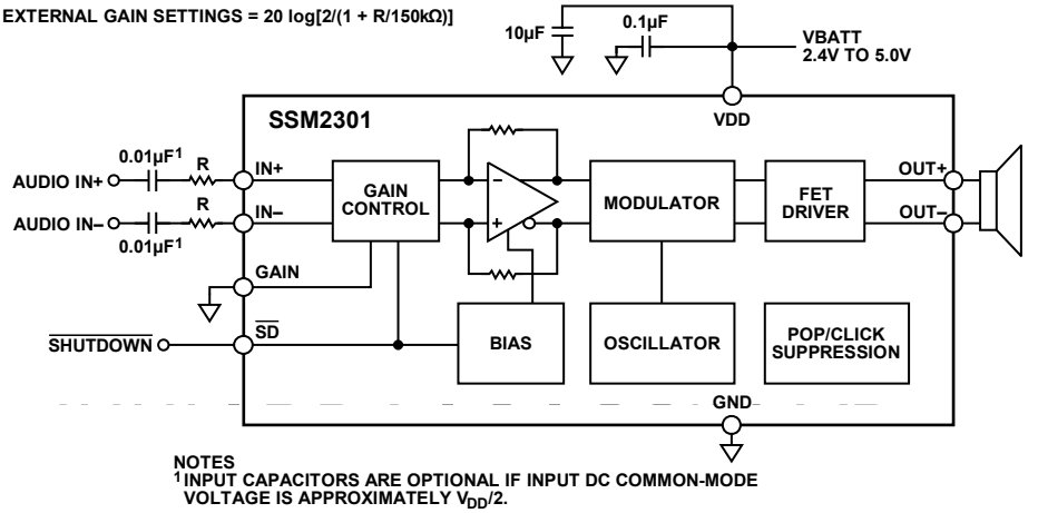
Figure 28. Differential Input Configuration, User-Adjustable Gain
