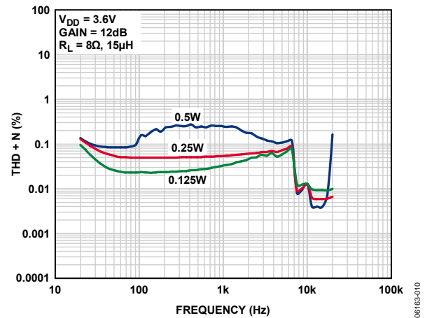
Figure 9. THD + N vs. Frequency, V_{DD} = 3.6V , A_v = 12dB , R_L = 8\Omega
