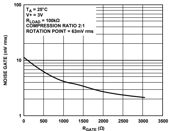
Figure 3. Noise Gate vs. R_{\text{GATE}}
