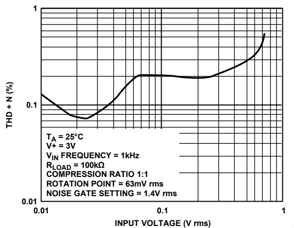
Figure 6. THD + N vs. Input
