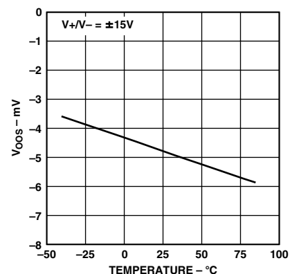
TPC 14. V_{00s} vs. Temperature
