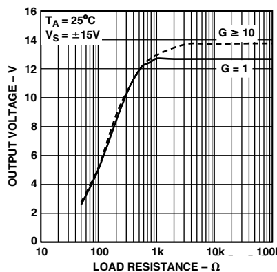
TPC 6. Output Voltage vs. Load Resistance
