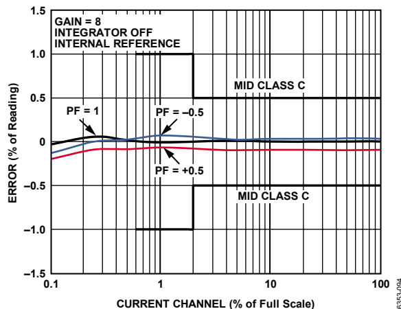
Figure 19. Active Energy Error as a Percentage of Reading (Gain = 8) over Power Factor with Internal Reference, Integrator Off
