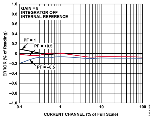
Figure 20. Reactive Energy Error as a Percentage of Reading (Gain = 8) over Power Factor with Internal Reference, Integrator Off
