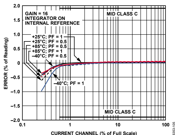
Figure 30. Current RMS Error as a Percentage of Reading (Gain = 16) over Power Factor with Internal Reference, Integrator On
