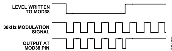
Figure 115. 38 kHz Modulation
