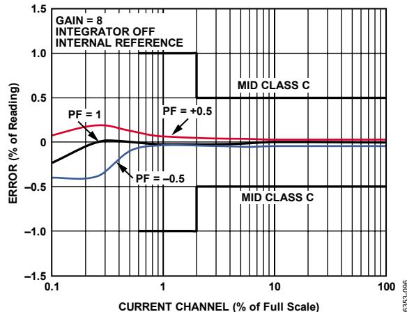
Figure 21. Current RMS Error as a Percentage of Reading (Gain = 8) over Power Factor with Internal Reference, Integrator Off
