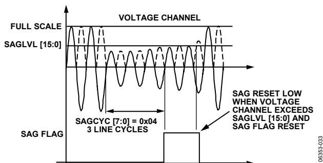
Figure 56. SAG Detection
