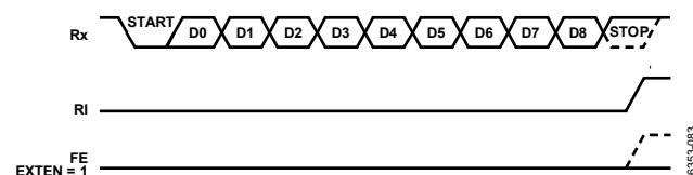
Figure 107. UART Timing in Mode 2 and Mode 3
