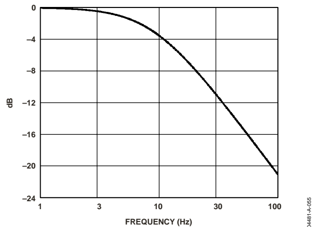
Figure 54. Frequency Response of LPF2
