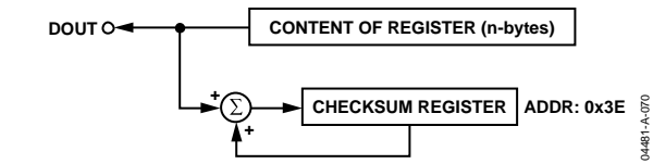
Figure 79. Checksum Register for Serial Interface Read
