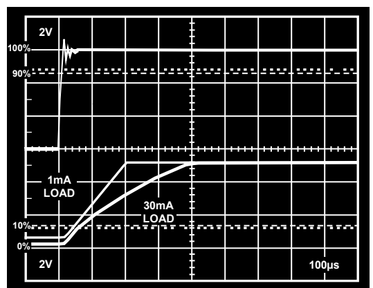
Figure 14. Power-On Response Time
