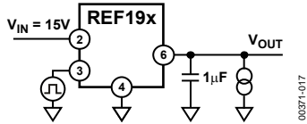
Figure 17. \overline{SLEEP} Response Time Measurement Circuit
