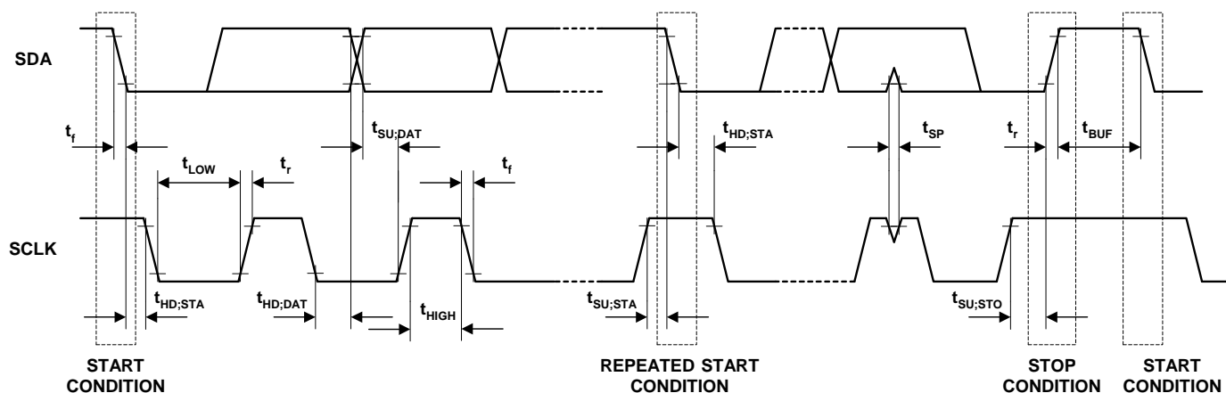
Figure 2. I 2 C Compatible Interface Timing
