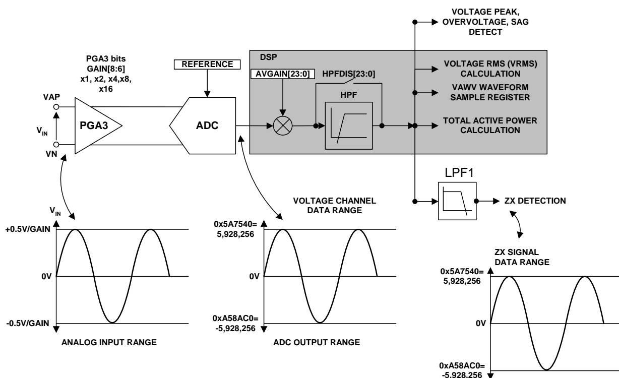
Figure 22. Voltage Channel Data Path
