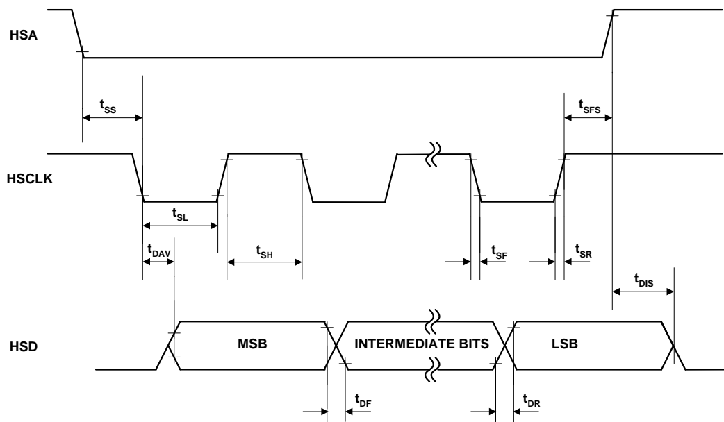
Figure 4. HSDC Interface Timing
