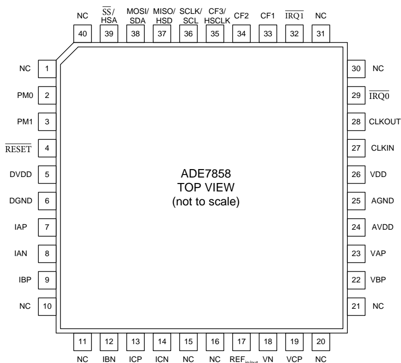
Figure 6. ADE7858 Pin Configuration
