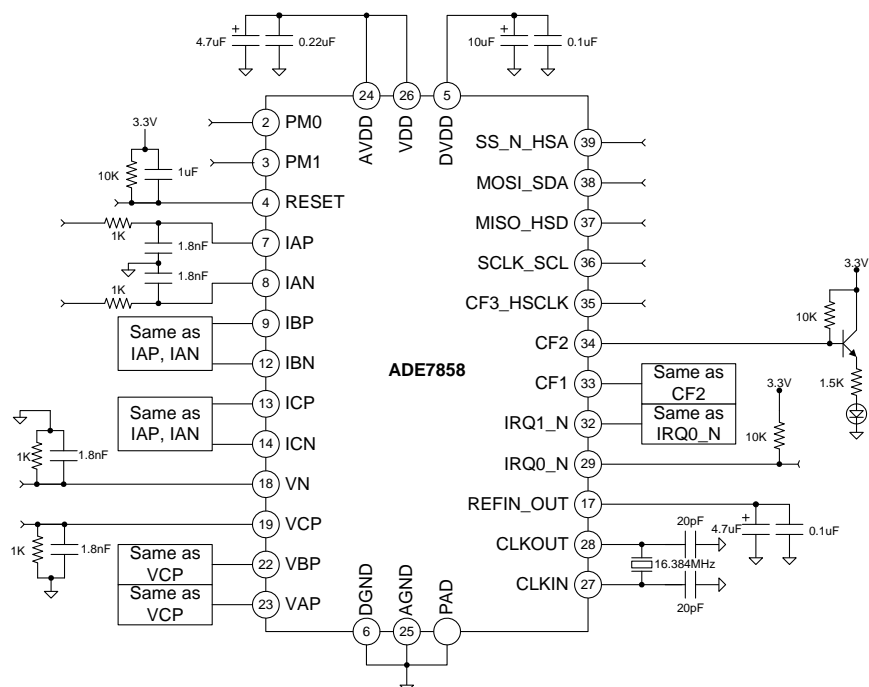
Figure 7. Test Circuit
