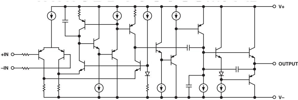
Figure 1. Simplified Schematic
