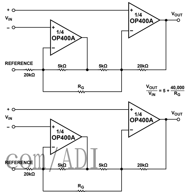
Figure 30. Dual Low Power Instrumentation Amplifier
