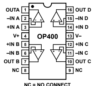
Figure 2. 16-Pin SOIC (S-Suffix)
