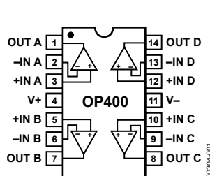
Figure 1. 14-Pin Ceramic DIP (Y-Suffix) and 14-Pin Plastic DIP (P-Suffix)
