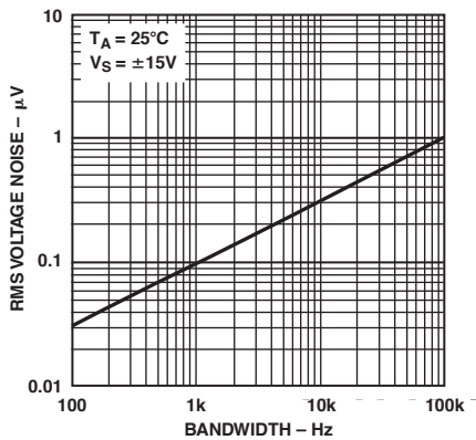
TPC 4. Input Wideband Voltage Noise vs. Bandwidth (0.1 Hz to Frequency Indicated)
