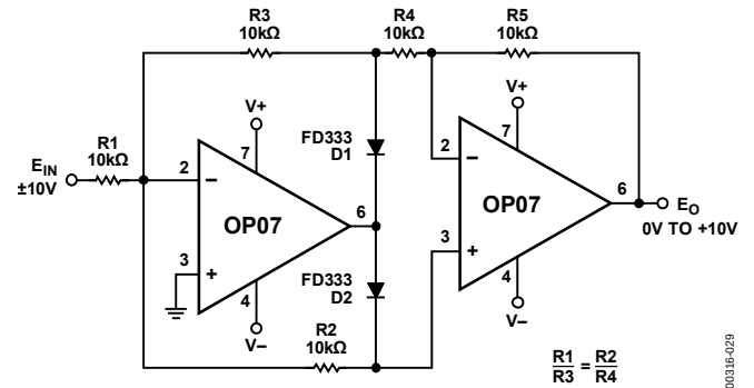
Figure 29. Burn-In Circuit
