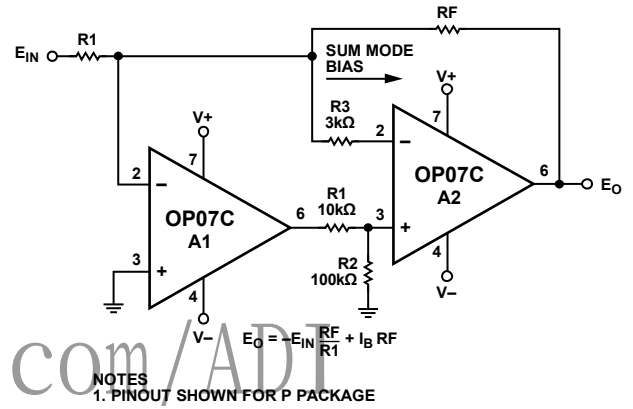
Figure 30. High Speed, Low V_{OS} Composite Amplifier
