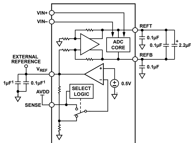
Figure 67. Internal Reference Configuration
