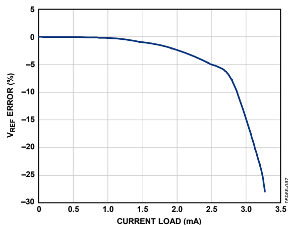
Figure 69. V_{REF} Accuracy vs. Load
