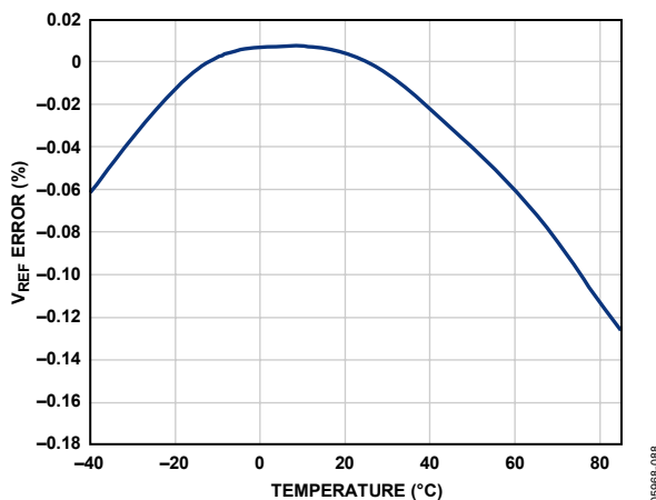
Figure 70. Typical V_{REF} Drift
