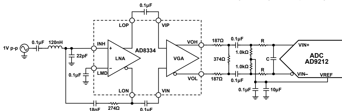
Figure 49. Single-Ended Input Configuration
