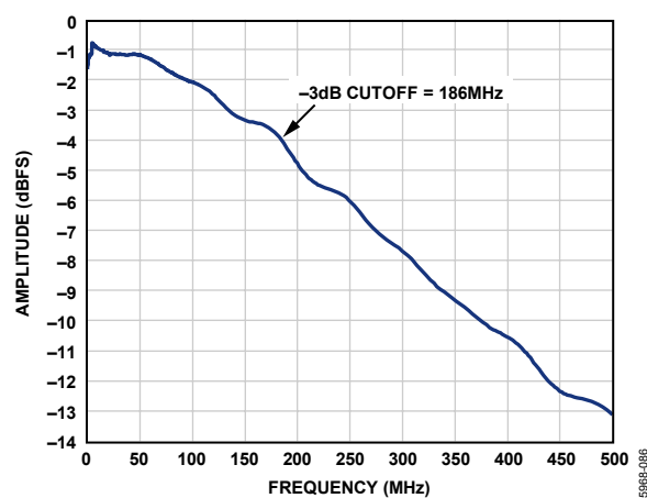
Figure 75. Evaluation Board Full Power Bandwidth
