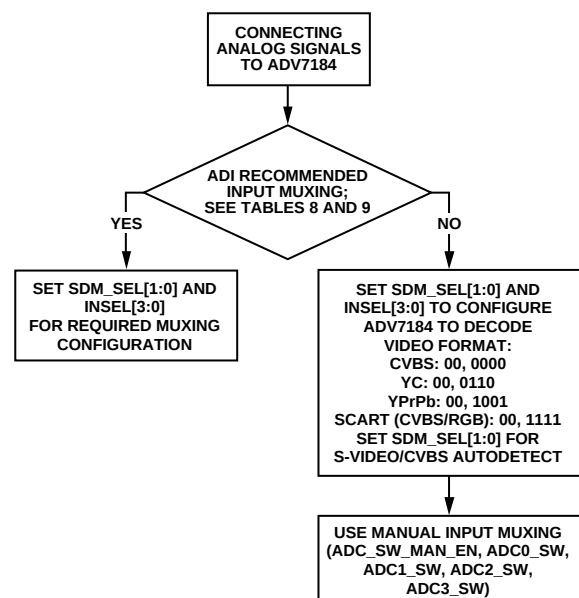
Figure 7. Input Muxing Overview
