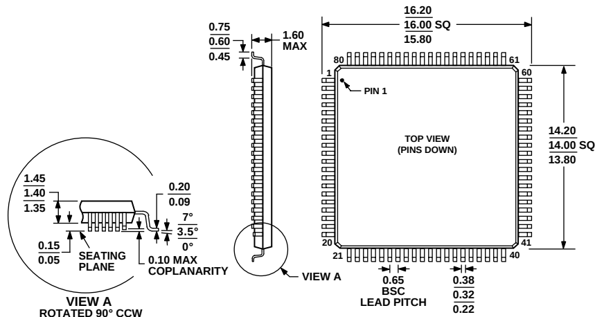
COMPLIANT TO JEDEC STANDARDS MS-026-BEC Figure 51. 80-Lead Low Profile Quad Flat Package [LQFP] (ST-80-2) Dimensions shown in millimeters
