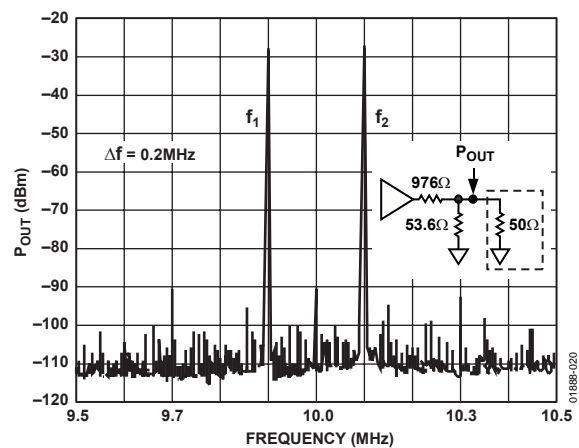
Figure 20. Intermodulation Distortion vs. Frequency
