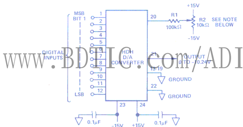
Figure 6. Noninverting Unipolar or Bipolar Voltage Output — HDS-1025
