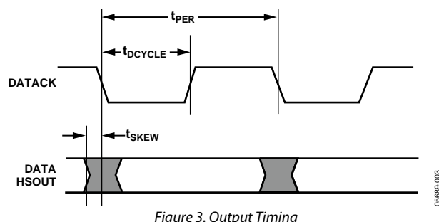
Figure 3. Output Timing
