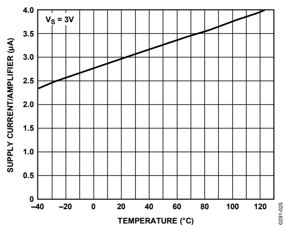
Figure 25. Supply Current/Amplifier vs. Temperature
