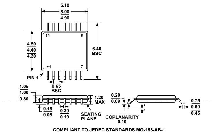
Figure 49. 14-Lead Thin Shrink Small Outline Package [TSSOP] (RU-14)
