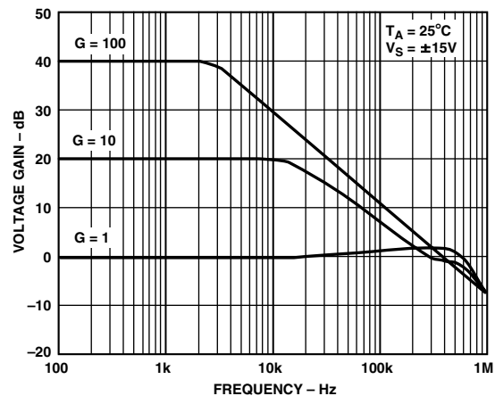
Figure 28. Closed-Loop Voltage Gain vs. Frequency
