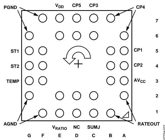
Figure 3. Pin Configuration
