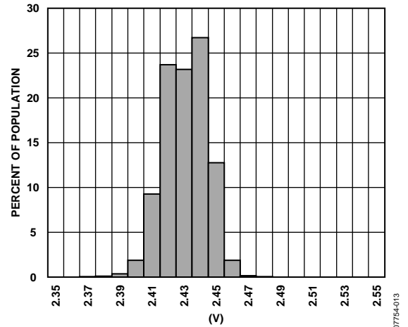
Figure 13. V_{TEMP} Output at 25°C ( V_{RATIO} = 5\text{ V} )
