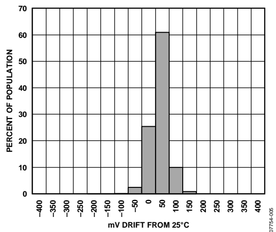
Figure 5. Null Drift over Temperature ( V_{\text{RATIO}} = 5 \text{ V} )
