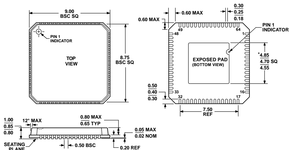
Figure 3. 64-Lead Lead Frame Chip Scale Package [LFCSP_VQ] 9 mm × 9 mm Body, Very Thin Quad (CP-64-1)
