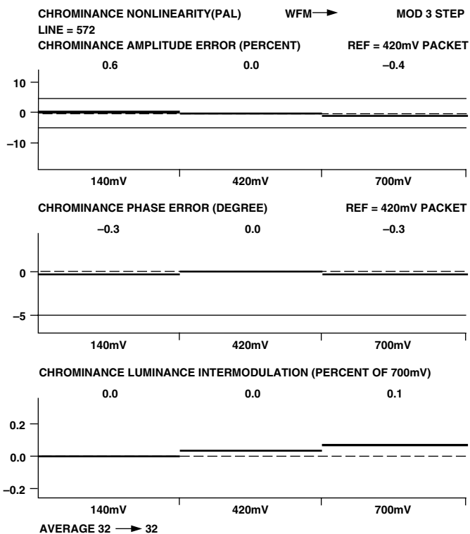
Figure 141. PAL Chrominance Nonlinearity
