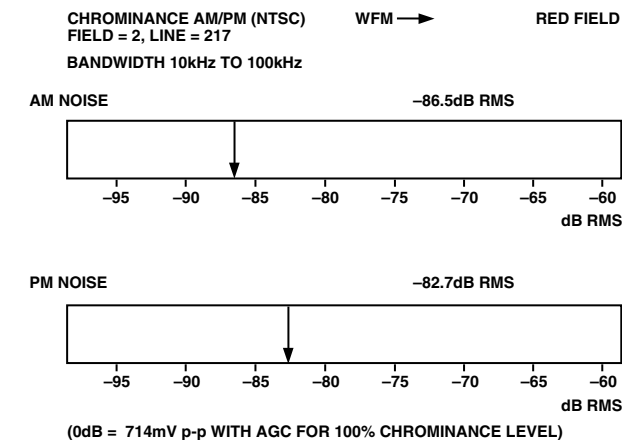
Figure 140. NTSC Chrominance AM/PM
