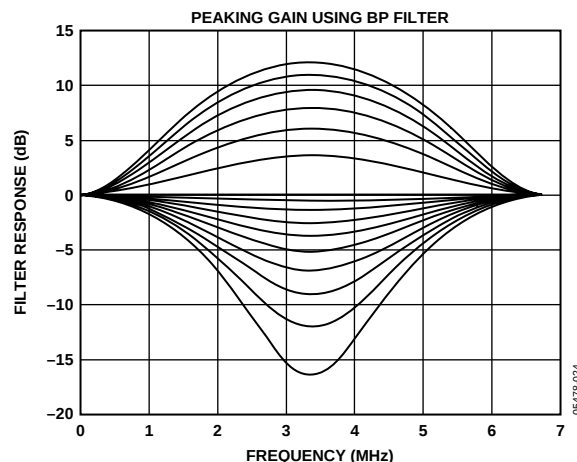
Figure 24. Peaking Filter Responses
