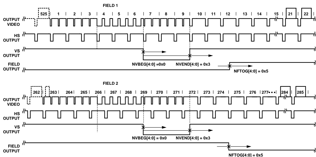
Figure 22. NTSC Typical Vsync/Field Positions Using Register Writes in Table 56
