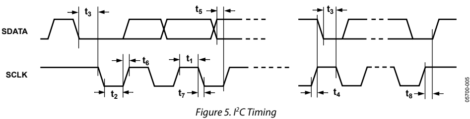
Figure 5. I 2 C Timing
