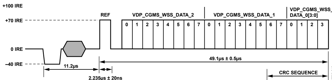
Figure 44. CGMS Waveform
