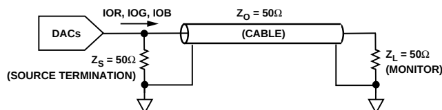
Figure 10. DAC Output Termination (Doubly Terminated 50 Ω Load)
