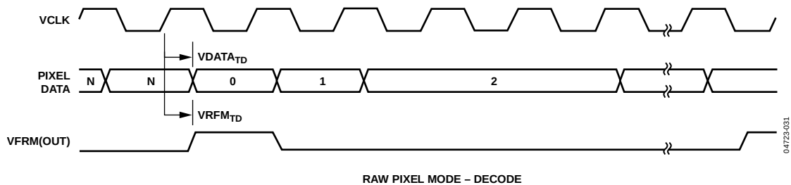
Figure 22. Raw Pixel Mode Timing
