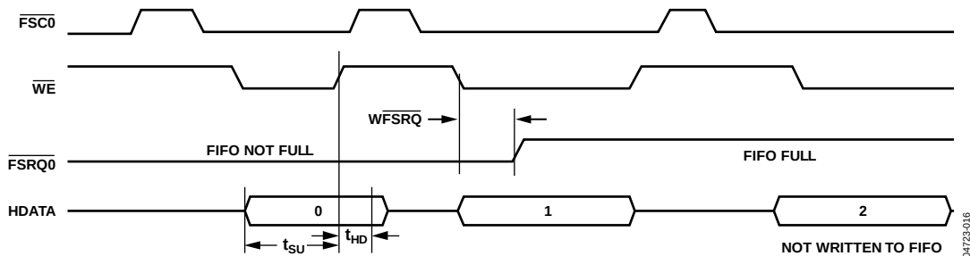
Figure 8. DCS DMA Mode—Single Write Access (Rev. 0.1 and Higher)
