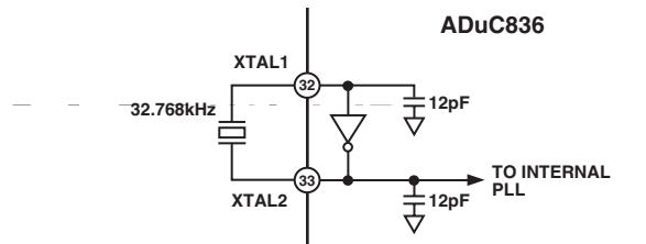
Figure 65. External Parallel Resonant Crystal Connections Other Hardware Considerations
