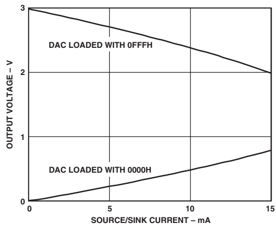
Figure 24. Source and Sink Current Capability with V_{REF} = V_{DD} = 3\text{ V} To reduce the effects of the saturation of the output amplifier at values close to ground and to give reduced offset and gain errors, the internal buffer can be bypassed. This is done by setting the DBUF bit in the CFG831 register. This allows a full rail-to-rail output from the DAC which should then be buffered externally using a dual supply op-amp in order to get a rail-to-rail output. This external buffer should be located as near as physically possible to the DAC output pin on the PCB. Note the unbuffered mode only works in the 0 to V_{REF} range.
