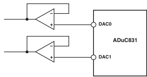
Figure 25. Buffering the DAC Outputs
