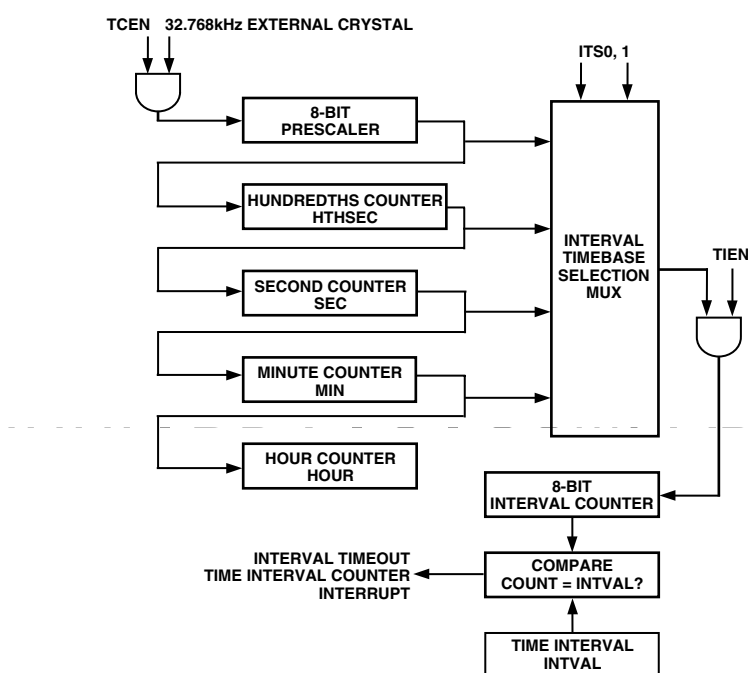
Figure 32. TIC, Simplified Block Diagram
