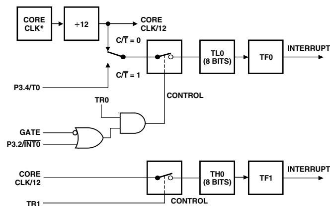
Figure 37. Timer/Counter 0, Mode 3
