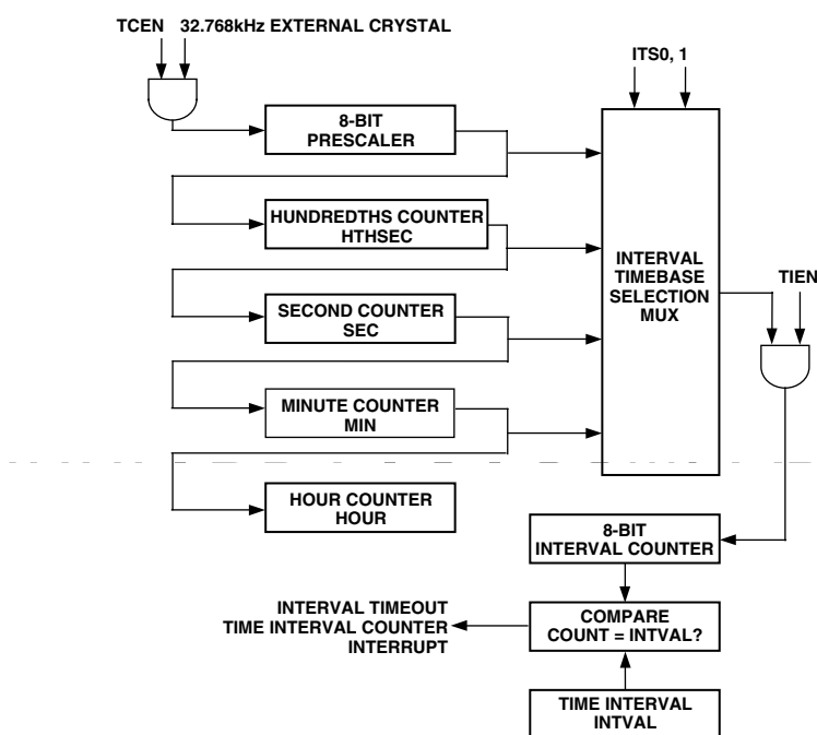
Figure 31. TIC, Simplified Block Diagram
