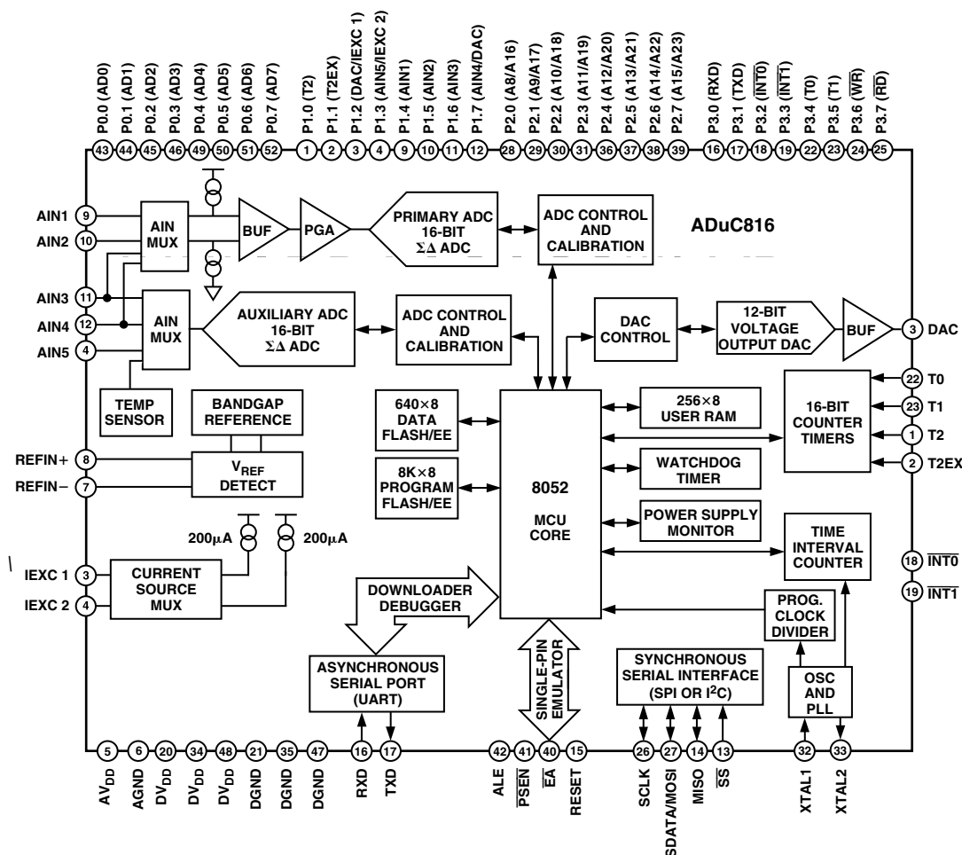
Figure 12. Block Diagram
