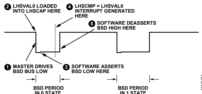
Figure 56. Master Read, Slave Transmit
