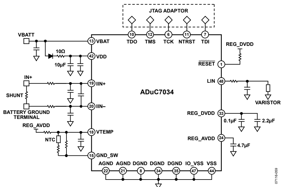
Figure 57. Schematic
