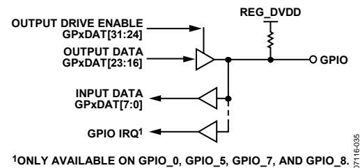
Figure 37. ADuC7034 GPIO
