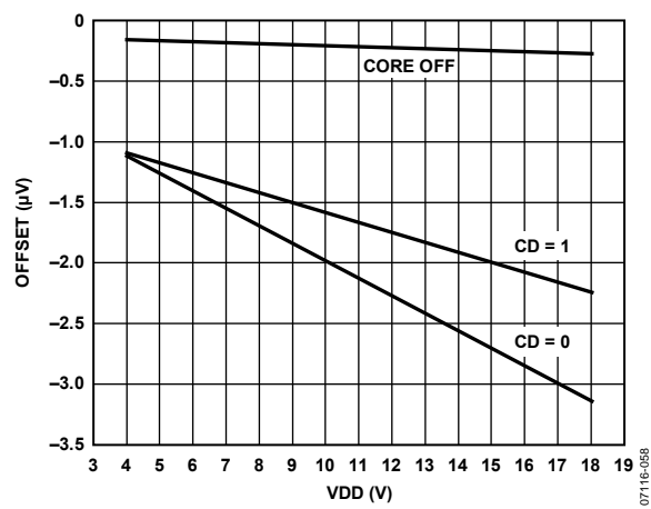
Figure 10. ADC Current Channel Offset vs. Supply @ 25°C
