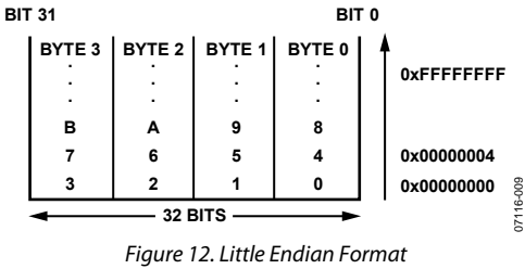
Figure 12. Little Endian Format
