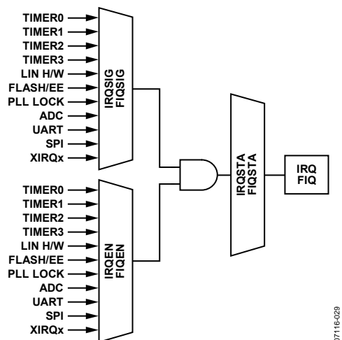
Figure 31. Interrupt Structure
