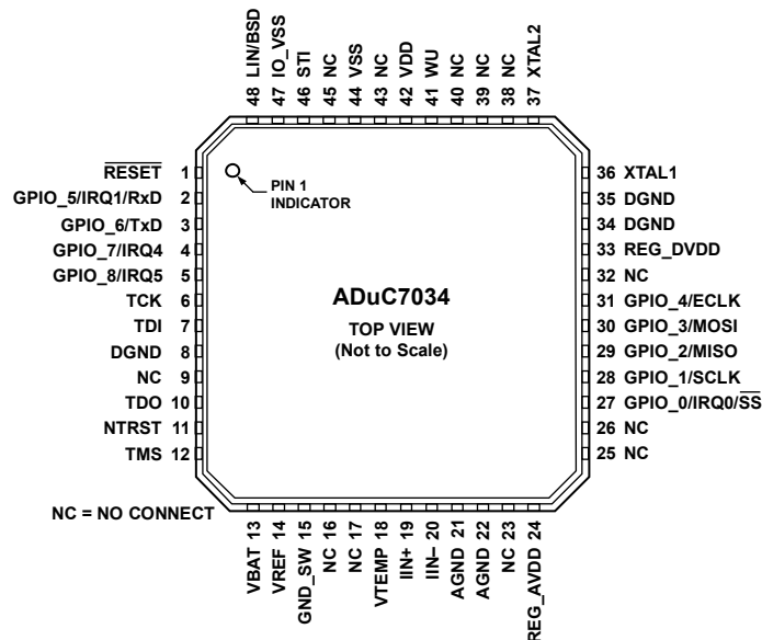
Figure 7. Pin Configuration
