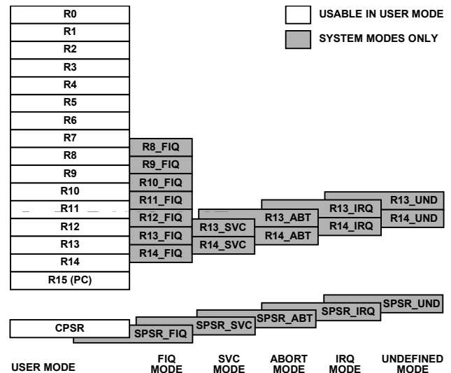
Figure 11. Register Organization
