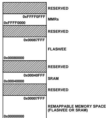
Figure 13. ADuC7033 Memory Map
