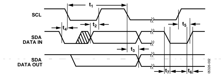
Figure 2. SMBus/I 2 C Timing Diagram
