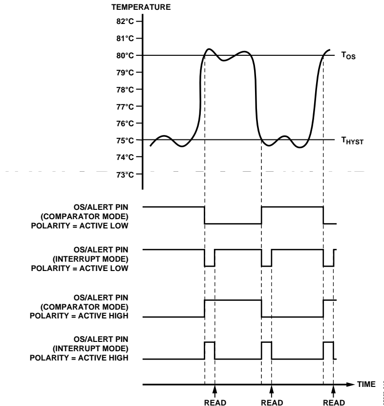
Figure 19. OS/ALERT Output Temperature Response Diagram
